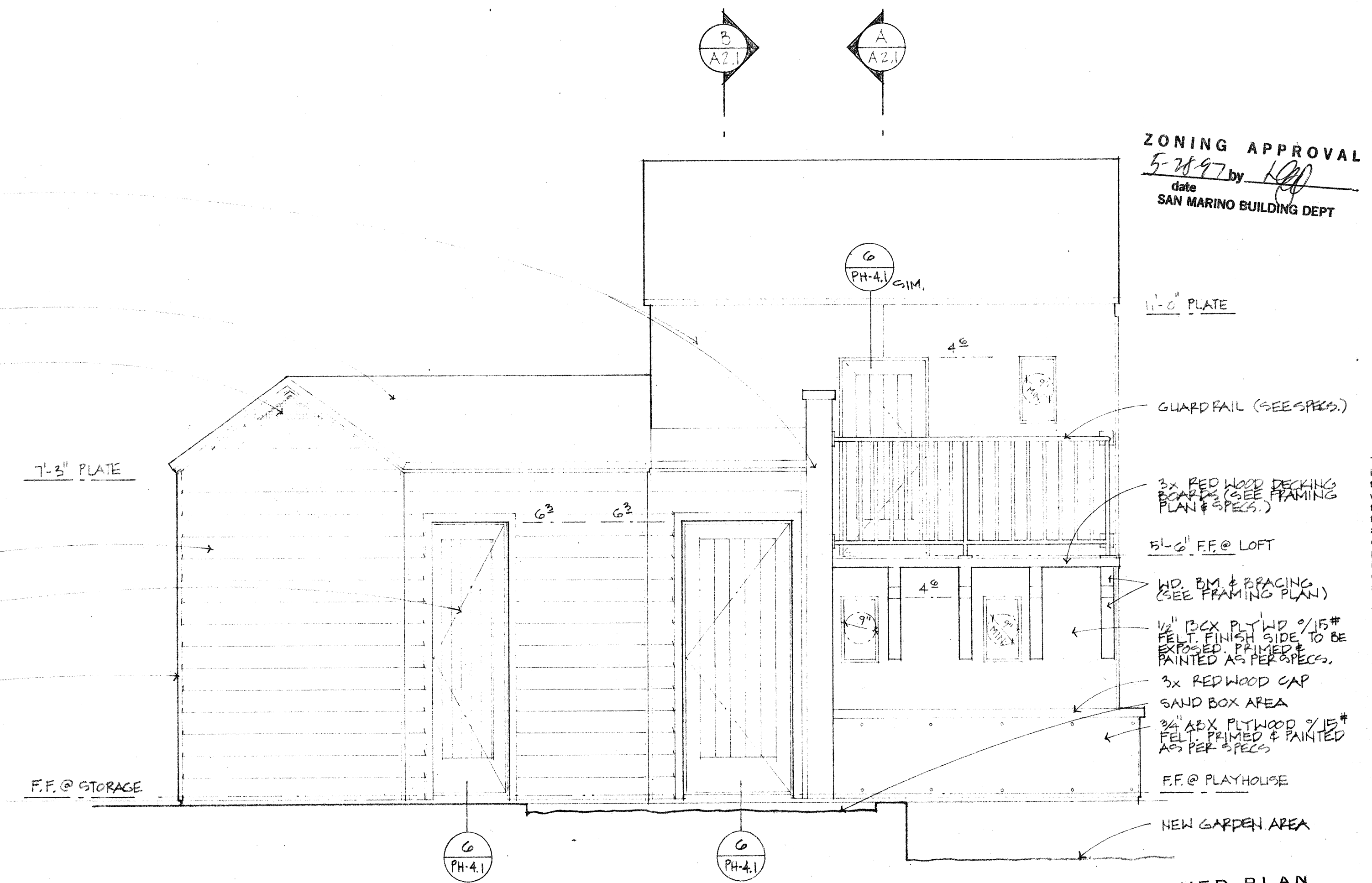
Southwest Elevation
