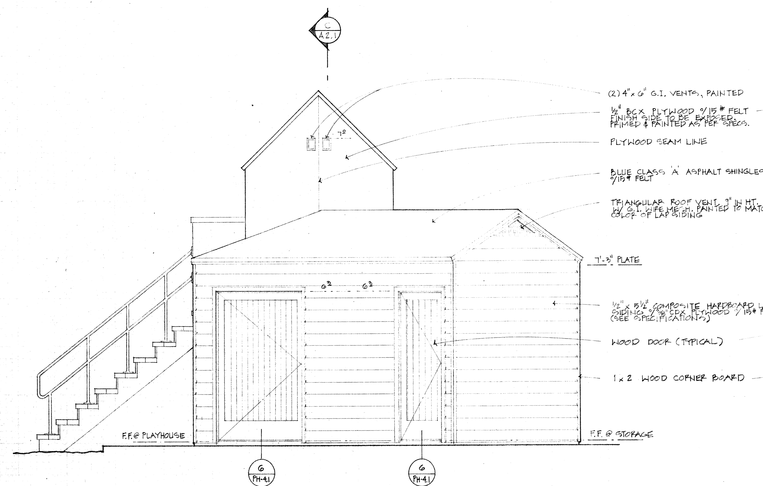
Northwest Elevation
