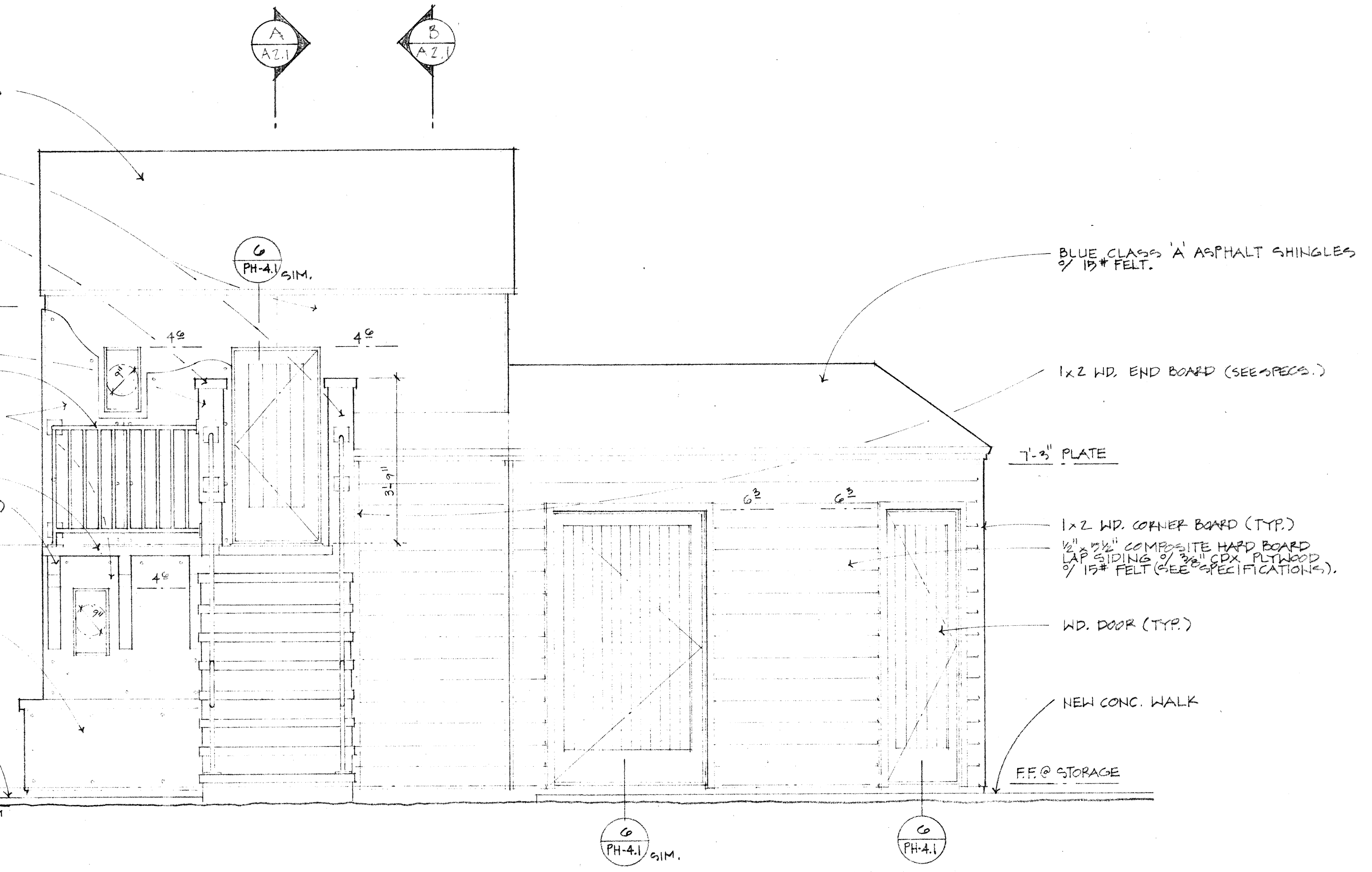
Northeast Elevation
